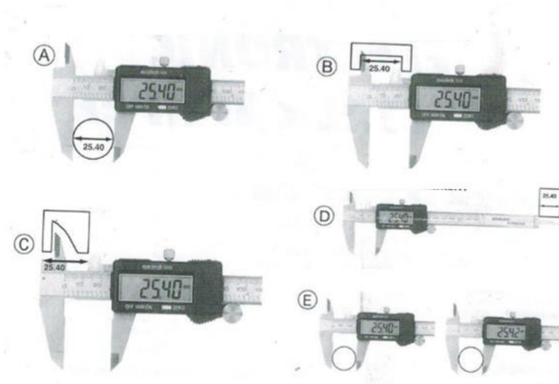
A) External measurement B) Internal measurement C) Step measurement D) Depth measurement E) Differential measurement
